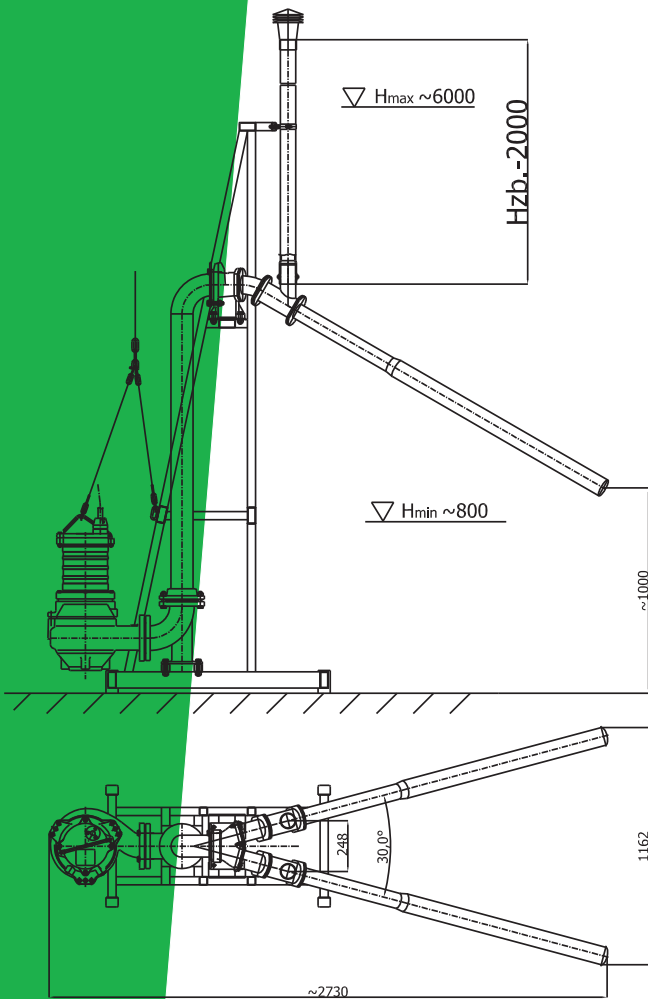
Strumienica S2S-44S;-54S; -74S; -94S; -114S
